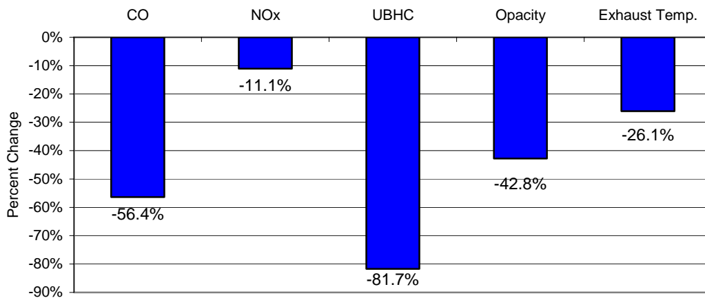
Figure 5: Effect of EnviroFuels DFC on Emissions
